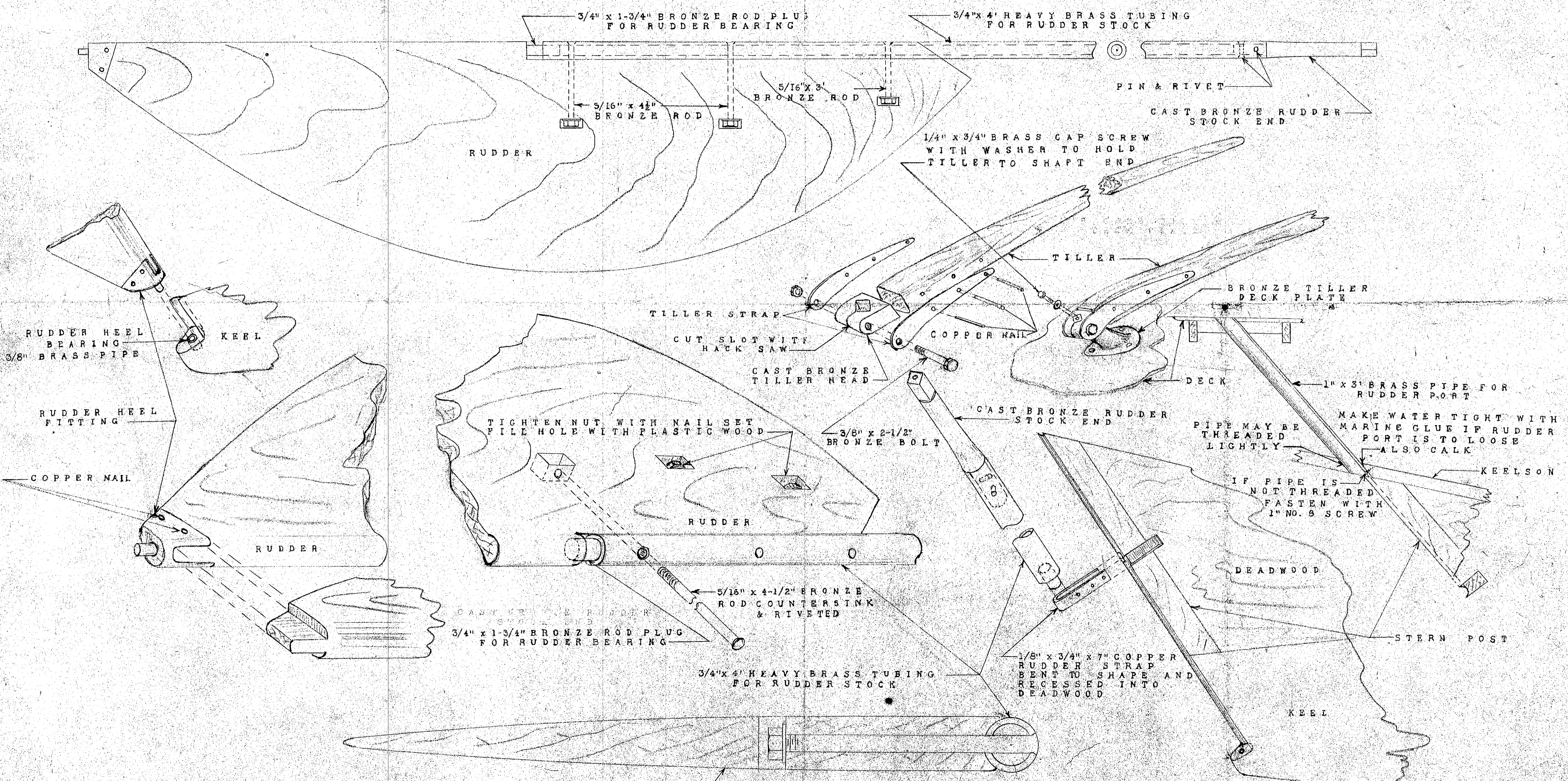
MERCURY CLASS RUDDER DETAIL PLAN DESIGNED BY ERNEST NUNES
