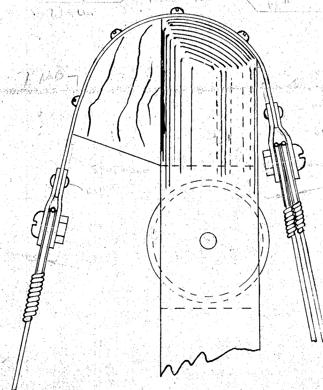
DETAIL OF MAST HEAD
