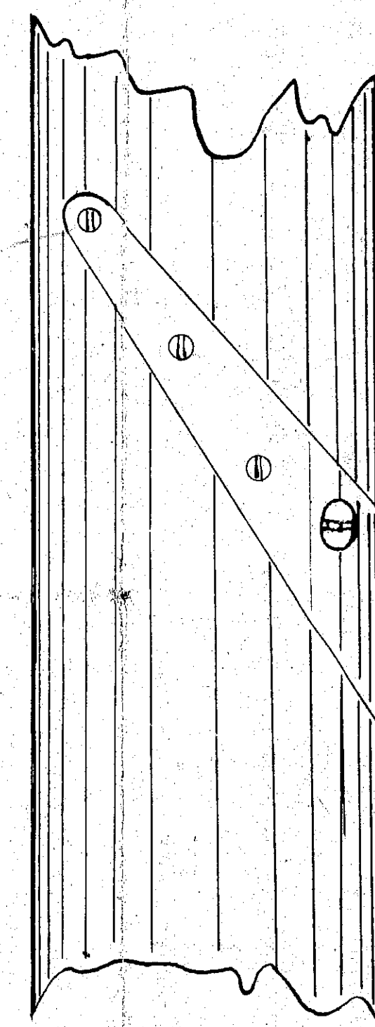
Expanded pattern 14# Brass 2 required
